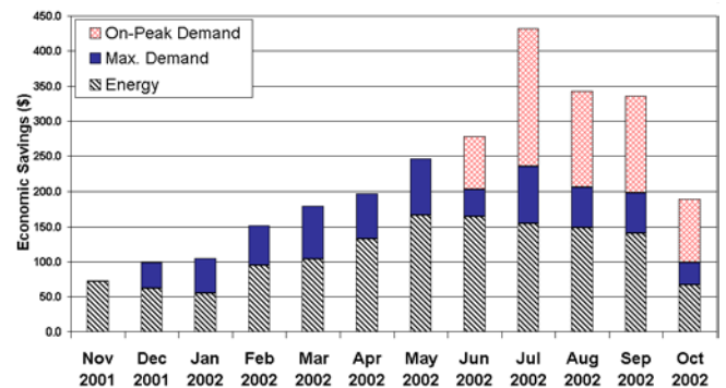
Figure 6 Economic Savings Associated with Solar Photovoltaic System
