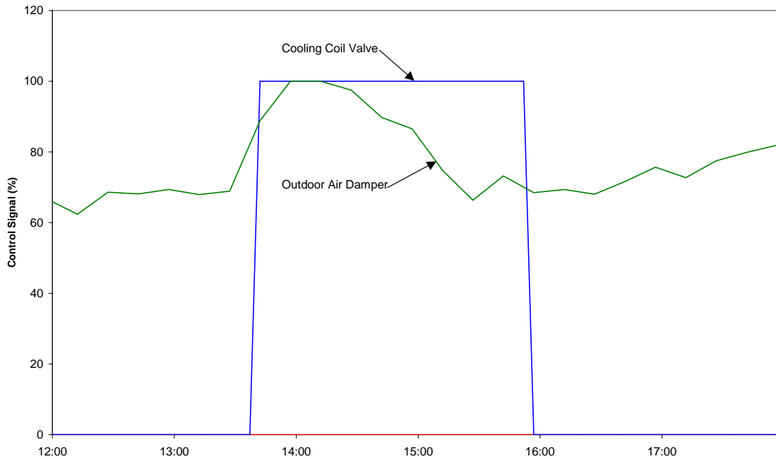
Figure 5.21. Simultaneous Mechanical Cooling and Economizing.
