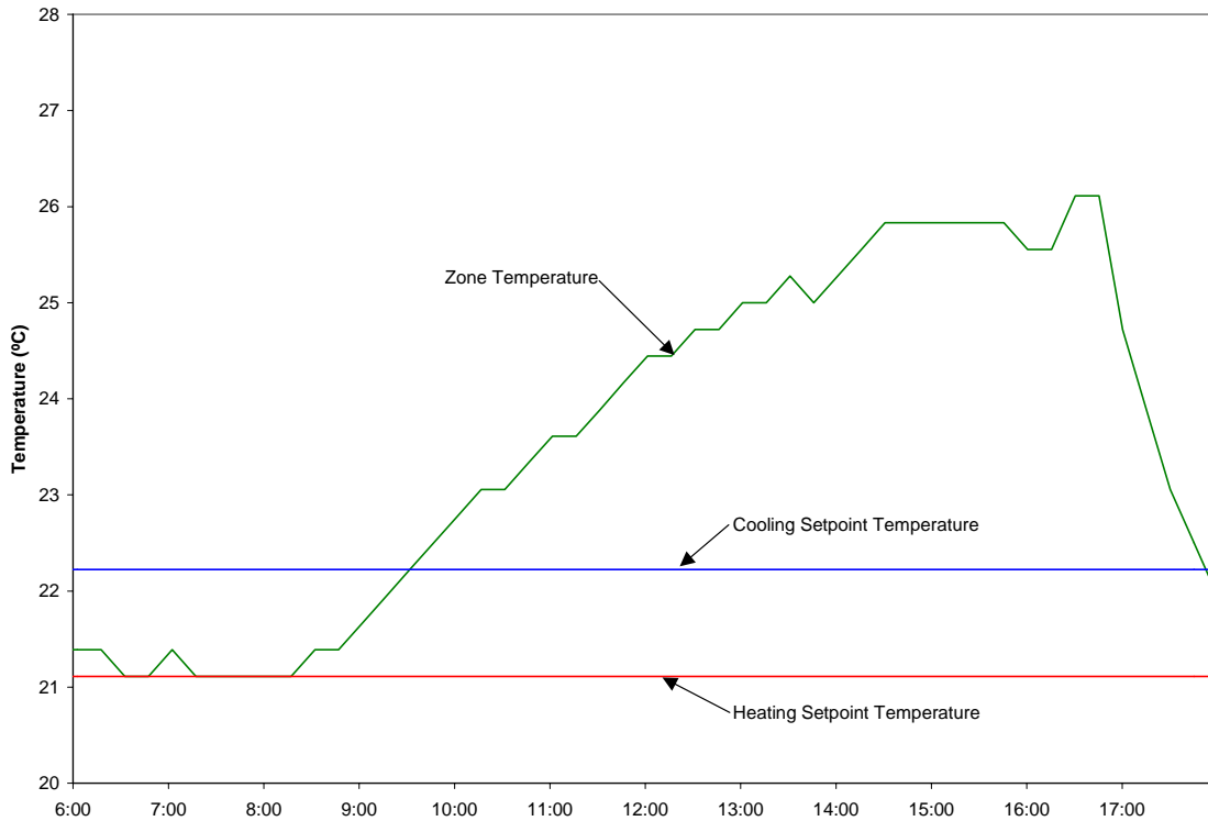
Figure 5.23. Undersized VAV Box.
