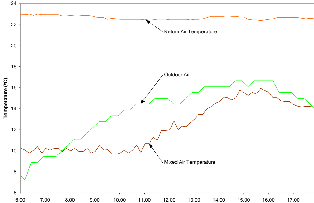
Figure 5.22. Outdoor Air Temperature Sensor Error.
