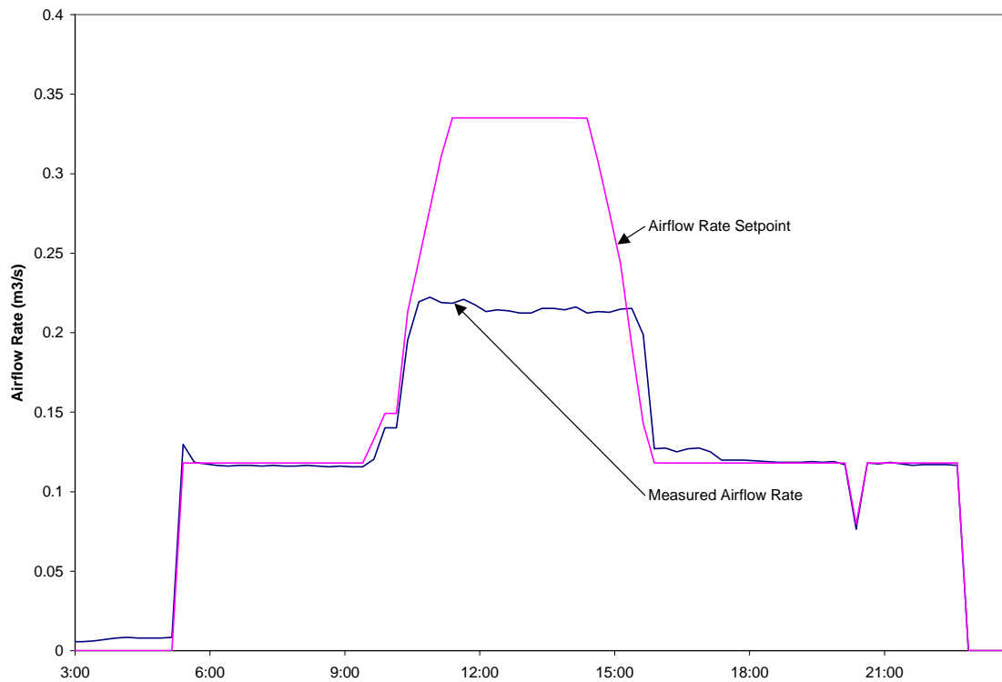
Figure 5.24. Undersized Supply Fan.
