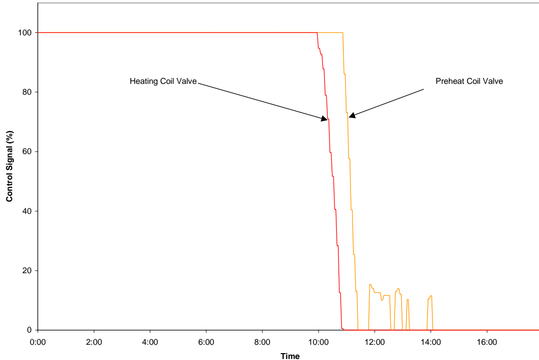
Figure 5.16. Hot Water Converter Offline.
