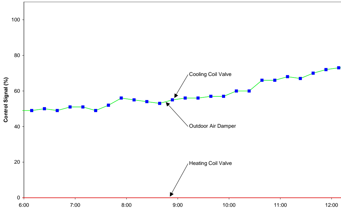
Figure 5.20. Simultaneous Mechanical Cooling and Economizing.
